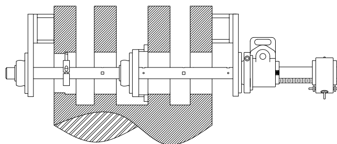
Line Boring
