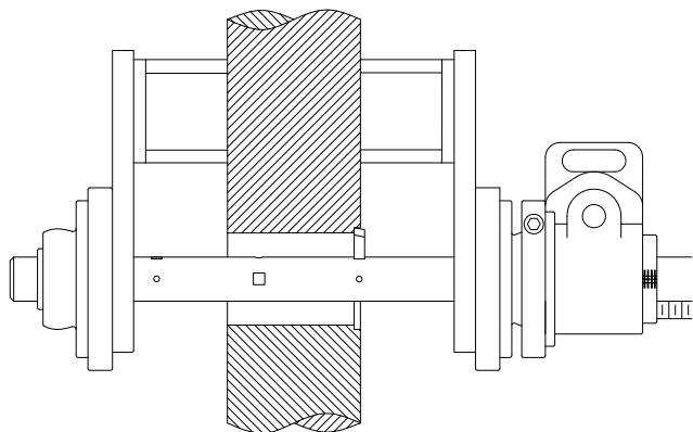
Conventional Boring
