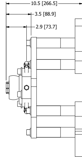
Universal bearing mount assembly (side view)
